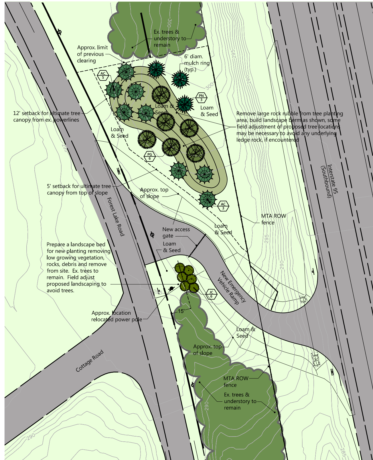
Landscape Plan - Emergency Vehicle Ramp Area
