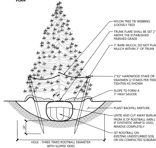
Evergreen Tree Planting 1/16 LD_604 N.T.S. Source: VHB
